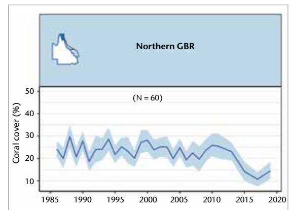
Figure 25. Trends in average hard coral cover for the northern Great Barrier Reef (GBR) based on manta-tow surveys up to June 2019. N indicates the number of reefs contributing to the analyses; blue shading represents 95% credible intervals. Note that many reefs in this region do not have a regular survey history and that in 2019 not all inshore reefs could be surveyed (Source: Australian Institute of Marine Science (AIMS)). 94
