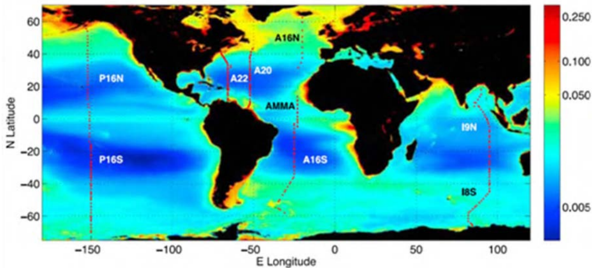
Fig. 5-3. Distribution of CDOM absorption coefficients at 443 nm from satellite ocean colour observations derived from Global System for Mobile Communications (GSM) satellite retrieval of merged SeaWiFS and MODIS Aquadata. 148, 199 Field observations collected on meridional transects showed that UV absorption coefficients at 325 nm were approximately 10-fold greater than absorption coefficients at 443 nm. The increase in CDOM concentrations towards the poles reflects, in part, decreased photobleaching as surface UV irradiance decreases (Fig. 1 from Nelson et al. 148 ).
