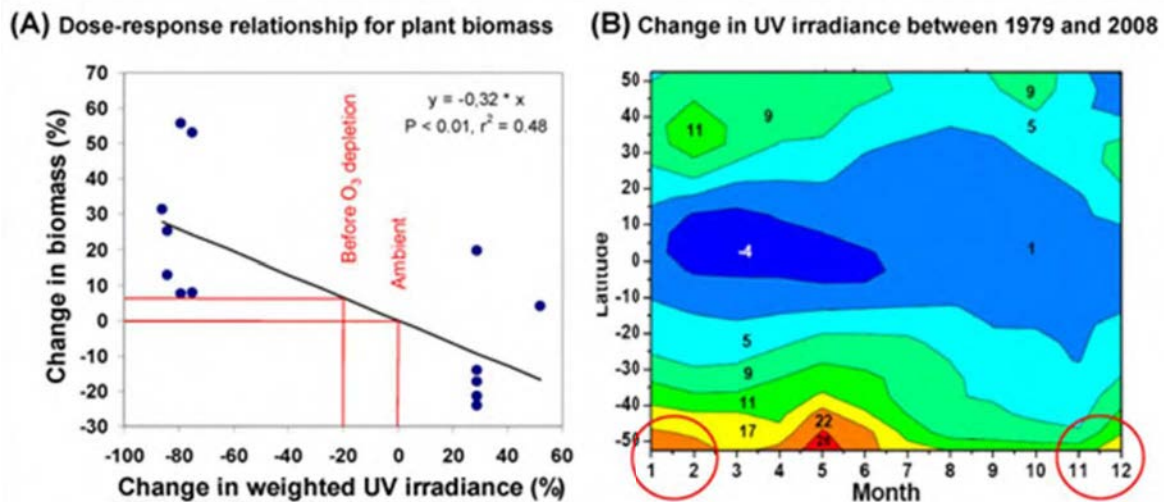
Fig. 3-1. A quantitative estimate of the reduction in the growth of the primary producers that may have occurred as a consequence of increased UV-B radiation between 1979 and 2008. (A) Change in aboveground biomass as a function of experimentally-imposed changes in weighted UV irradiance. The growth data are derived from a meta-analysis of field studies in high-latitude ecosystems (which involved experimental attenuation or supplementation of ambient solar UV-B radiation), and are expressed as % change in relation to the growth of the plants receiving ambient solar radiation 102 . The UV doses are weighted using the generalised plant function 28 , and expressed as % change relative to the ambient level [Note that, for this function, a 10 % increase in UV corresponds to a 5% reduction in ozone; i.e., a RAF of 2 (see McKenzie et al. 97 ). The red lines focus on the example discussed in the text. For areas where ozone depletion over the last three decades has led to a 20 % increase in the summertime levels of weighted UV radiation (areas approximately designated by the red circles in panel B), the difference in plant growth between 1979 and the present would be 6% or less, given the slope of the dose-response relationship and assuming that all other factors are equal. (B) Percentage change in UV irradiance (numbers inside the coloured areas), weighted using the generalised plant function 28 , as a function of time of the year and latitude (between 55° S and 55° N), between 1979 and 2008 (data from Herman 59 ). Note that the relative changes in weighted UV irradiance at 50° to 55° S are much greater near the winter solstice, but the absolute irradiance levels are very low during the winter and vegetation is less physiologically active and possibly snow-covered at that time of year.
