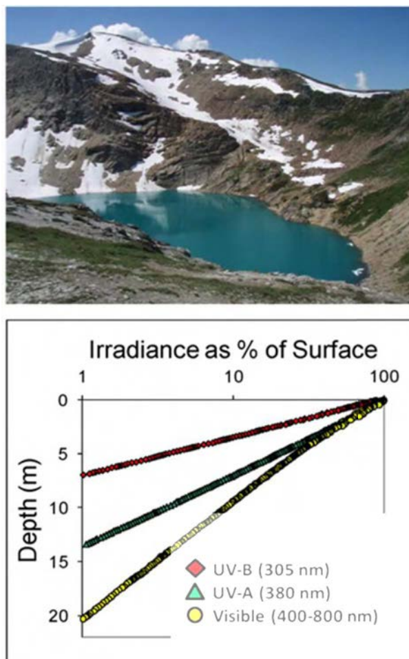
Fig. 4-2. Profiles of UV-B, UV-A radiation, and visible light penetration in Sunlite Lake, an alpine lake in the Canadian Rocky Mountains. The high elevation of alpine lakes leads to high incident UV radiation, while the low levels of DOM in alpine lakes lead to high UV transparency of the waters. The result is that aquatic organisms are exposed to higher levels of damaging UV radiation in alpine lakes than in any other aquatic ecosystem.
